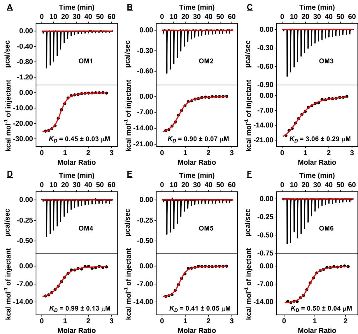
Figure S16. Characterization of oxycodone binding affinity of six aptamer candidates using ITC. The top panels display the heat generated from each titration of oxycodone into (A) OM1, (B) OM2, (C) OM3, (D) OM4, (E) OM5 and (F) OM6. Bottom panels show the integrated heat of each titration after correcting for the heat of dilution of the titrant.
