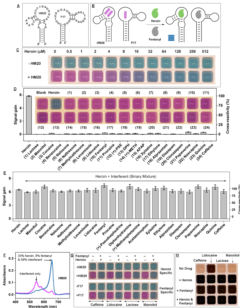
Figure 4. Detection of heroin and fentanyl using aptamer-based dye-displacement assays. (A) Secondary structures of HM20 and F17 based on NUPACK predictions. (B) Scheme of the dye-displacement assay using HM20, F17, and MTC (purple bars indicate monomeric/dimeric forms of the dye; blue bars indicate J -aggregates). (C) Photographs taken 5 min after addition of various concentrations of heroin to solutions of MTC alone (–HM20) or HM20-MTC complexes (+HM20). (D) Signal gain and cross-reactivity of the displacement assay to various interferents relative to the response to heroin. Photographs of samples were taken 5 min after adding mixtures of 25 μM heroin and 50 μM interferent to HM20-MTC complexes. (E) Detection of heroin in binary mixtures of 25 μM heroin (~33%) with 50 μM interferent (~67%). (F) Absorbance spectra of HM20-MTC complexes in the presence of a 33:8:59 mixture of heroin, fentanyl, and an interferent (caffeine, lidocaine, lactose, or mannitol) as well as each interferent alone. These spectra overlap for all four drug mixtures and all four interferent samples. (G) Photographs of the dye-displacement assays analyzed in panel F (top) as well as equivalent assays performed with the fentanyl-specific aptamer F17 (bottom). (H) Photographs of Marquis test results for interferent alone, binary mixtures containing heroin and interferent (33:67) or fentanyl and interferent (8:92), or ternary mixtures containing heroin, fentanyl, and interferent (33:8:59). Error bars represent the standard deviations of three independent experiments.
