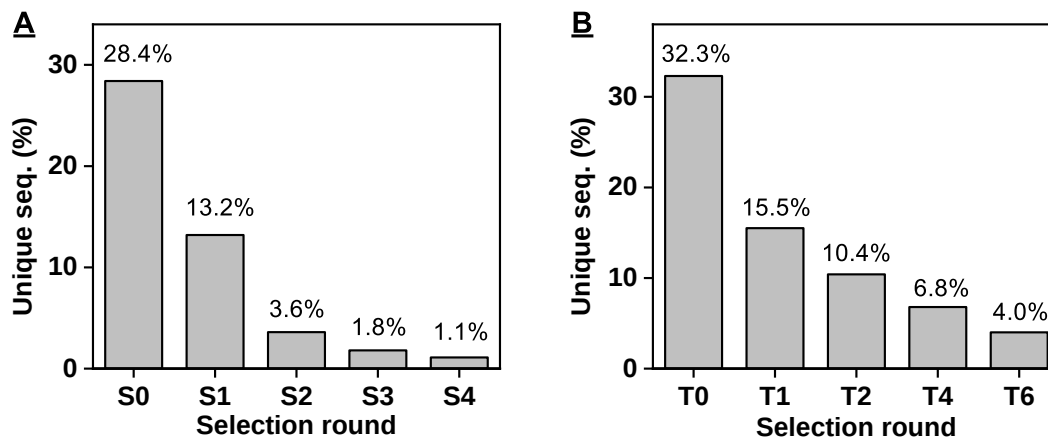
Figure S8. Percent of unique sequences from (A) HM serial SELEX rounds S0–4 and (B) OM toggle SELEX rounds T0, T1, T2, T4 and T6.
