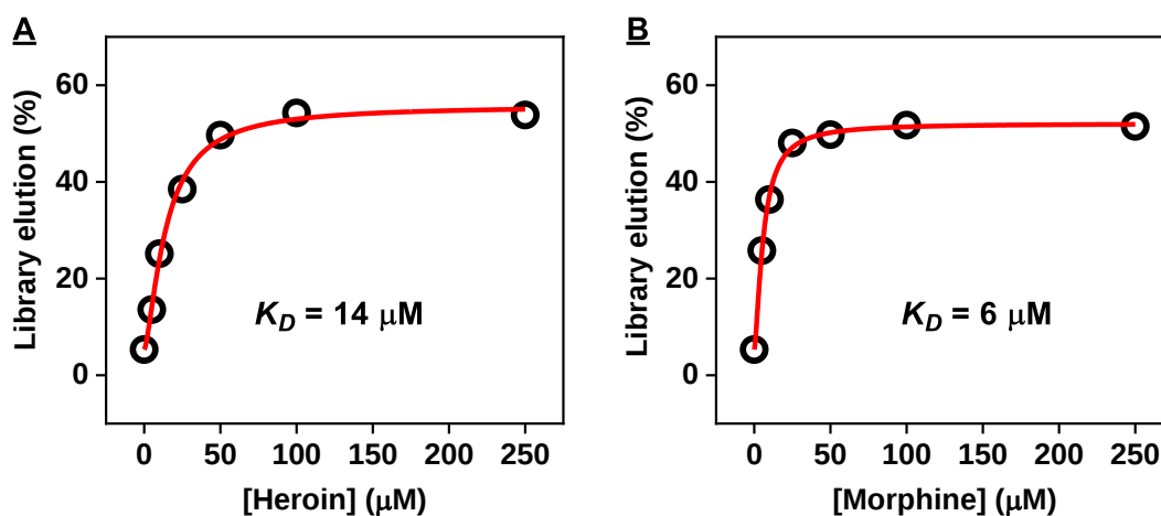
Figure S5. The binding affinity of the S4 pool for (A) heroin and (B) morphine. All fractions were PCR amplified and then analyzed via gel-elution assay. All binding curves were fitted with a modified one-site Langmuir equation to determine K_D .
