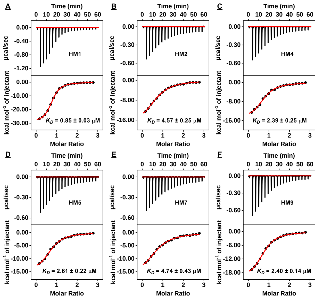
Figure S11. Characterization of morphine binding affinity of six aptamer candidates using ITC. The top panels display the heat generated from each titration of morphine into (A) HM1, (B) HM2, (C) HM4, (D) HM5, (E) HM7 and (F) HM9. Bottom panels show the integrated heat of each titration after correcting for the heat of dilution of the titrant.
