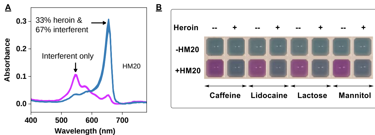
Figure S23. Detection of heroin using aptamer-based MTC-displacement assays. (A) Absorbance spectra of HM20-MTC complexes in the presence of a 33:67 mixture of heroin and interferent (caffeine, lidocaine, lactose, or mannitol) as well as each interferent alone. These spectra overlap for all four drug mixtures and all four interferent samples. (B) Photographs of the dye-displacement assays analyzed in panel A.
