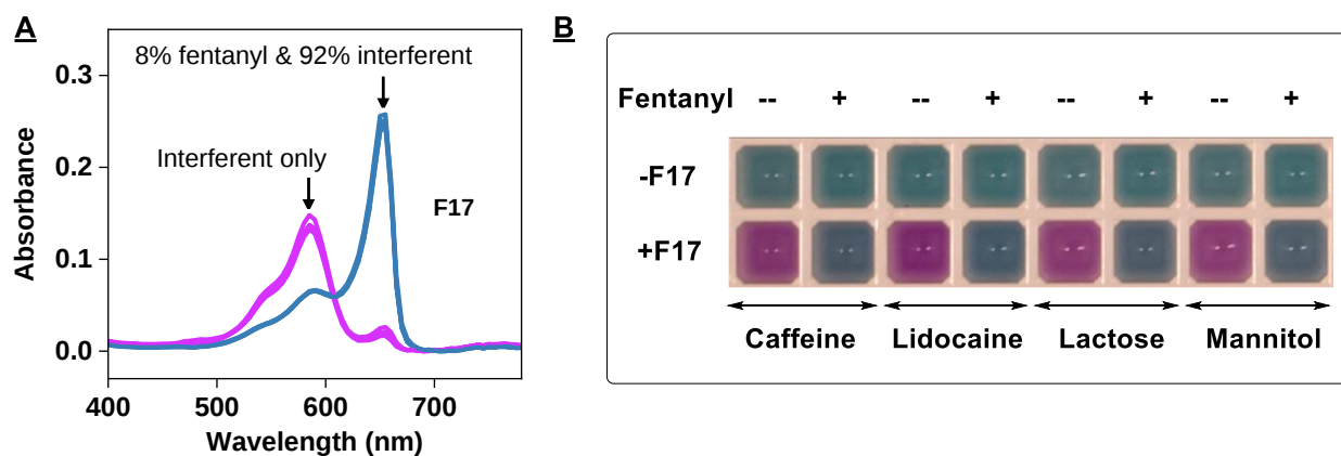
Figure S24. Detection of fentanyl using F17-based MTC-displacement assays. (A) Absorbance spectra of F17-MTC complexes in the presence of a 8:92 mixture of fentanyl and interferent (caffeine, lidocaine lactose, or mannitol) as well as each interferent alone. The spectra of F17-MTC complex overlap for all four drug mixtures and all four interferent samples. (B) Photographs of the dye-displacement assays for fentanyl detection using F17.
