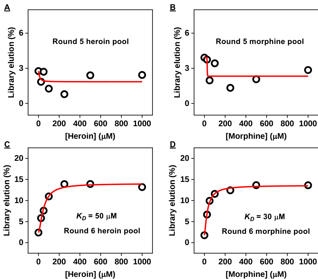
Figure S4. Binding affinity of the round P5 (A) heroin and (B) morphine pools and round P6 (C) heroin and (D) morphine pools. All fractions were PCR amplified and then analyzed via gel-elution assay. All binding curves were fitted with a modified one-site Langmuir equation to determine K_D .
