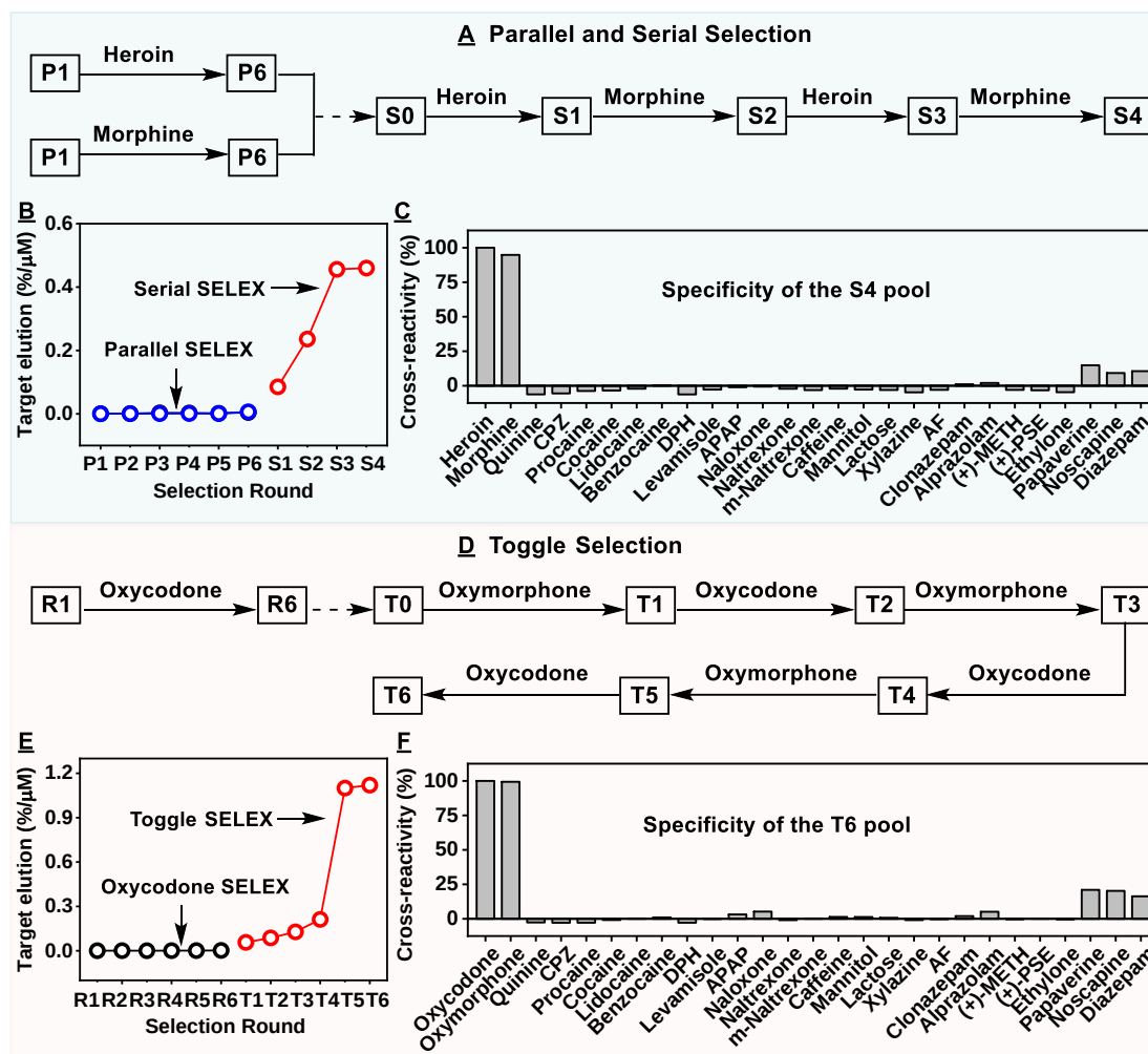
Figure S2. Isolation of opioid binding aptamers using library-immobilized SELEX. (A) Parallel and serial selection strategy for generating aptamers for morphine and heroin. (B) The percentage of pool eluted each round by target per micromolar concentration. Target for P1–P6 is heroin or morphine, and target for serial selection is either heroin or morphine. (C) Cross-reactivity of the round S4 pool against heroin, morphine and interferents. Cross-reactivity is calculated relative to heroin. (D) Toggle selection strategy for generating aptamers for oxycodone and oxymorphone. (E) The percentage of pool eluted each round by target per micromolar concentration. Target for R1–R6 is oxycodone and target for T1–T6 is either oxymorphone or oxycodone. (F) Cross-reactivity of the round T6 pool against oxycodone, oxymorphone and interferents. Cross-reactivity is calculated relative to oxycodone. In cross-reactivity assays, targets were tested at 25 \mu\text{M} and interferents were tested at a concentration of 250 \mu\text{M} , except for alprazolam, clonazepam, diazepam, which were tested at 100 \mu\text{M} in solutions containing 1% MeOH.
