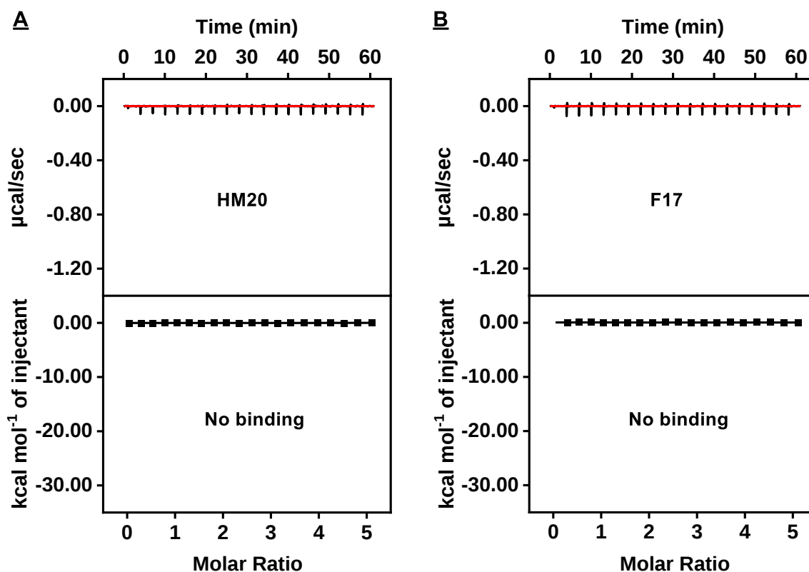
Figure S26. Isothermal titration calorimetry (ITC) measurements of the binding affinity of (A) heroin-binding aptamer HM20 to fentanyl and (B) fentanyl-binding aptamer F17 to heroin. The top panels present the raw data showing heat generated from each titration of target into the aptamers, and bottom panels depict the integrated heat of each titration after correcting for dilution heat of titrant. Data were fitted with a single-site binding model.
