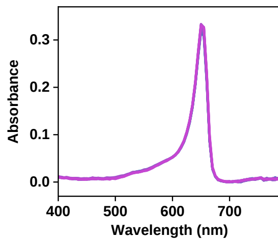
Figure S30. Effect of oxycodone on the absorbance spectrum of MTC alone. Spectra of 2.5 \mu\text{M} MTC in the presence of 0, 0.5, 1, 2, 4, 8, 16, 32, 64, 128, 256, and 512 \mu\text{M} oxycodone with no aptamer present, where the blue-to-purple color gradient represents increasing target concentrations.
