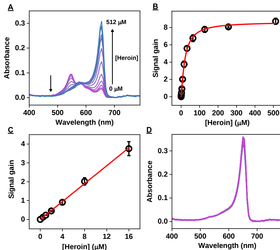
Figure S22. Detection of heroin using MTC and HM20. (A) Absorbance spectra of HM20-MTC complexes challenged with various concentrations of heroin, with the purple-to-blue-green color gradient representing increasing heroin concentration. (B) Calibration curve and (C) linear range of absorbance spectra of solutions containing 2.5 μM MTC and 6 μM HM20 challenged with 0, 0.5, 1, 2, 4, 8, 16, 32, 64, 128, 256, and 512 μM heroin. (D) Spectra of samples containing 2.5 μM MTC in the presence of 0, 0.5, 1, 2, 4, 8, 16, 32, 64, 128, 256, and 512 μM heroin, where blue-to-purple color gradient represents increasing target concentrations.
