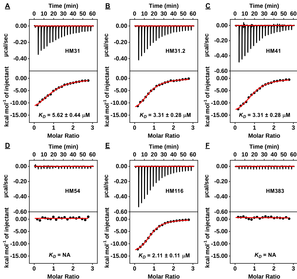
Figure S14. Characterization of morphine binding affinity of six aptamer candidates using ITC. The top panels display the heat generated from each titration of morphine into (A) HM31, (B) HM31.2, (C) HM41, (D) HM54, (E) HM116 and (F) HM383. Bottom panels show the integrated heat of each titration after correcting for the heat of dilution of the titrant.
