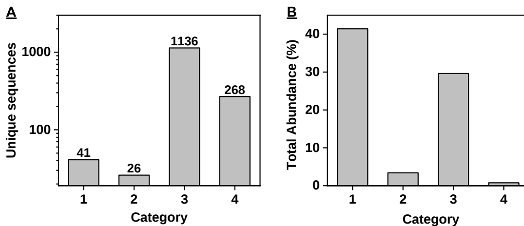
Figure S9. HTS analysis of the final S4 pool for heroin and morphine. (A) The number of unique sequences and (B) percent of the total pool belonging to each of the four categories described in the main text.
