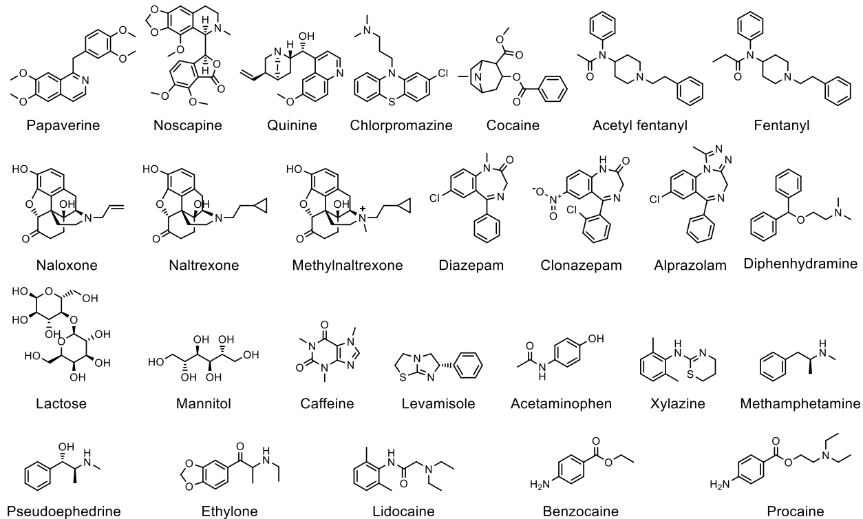
Figure S3. Chemical structure of interferents employed in counter-SELEX.
