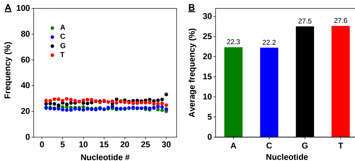
Figure S1. HTS analysis of randomized N30 library used for this work. (A) The frequency of the four nitrogenous bases at each nucleotide position of the random region. (B) The average frequency of each base at any given position in the random region.
