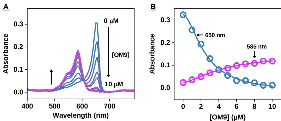
Figure S28. Binding of MTC to OM9. (A) Absorbance spectra of solutions containing 2.5 \mu\text{M} MTC with 0, 1, 2, 3, 4, 5, 6, 7, 8, 9 or 10 \mu\text{M} OM9, where the blue-to-purple color gradient shows increasing aptamer concentration. (B) Absorbance of MTC monomers at 585 nm and J-aggregates at 650 nm plotted versus concentration of OM9.
