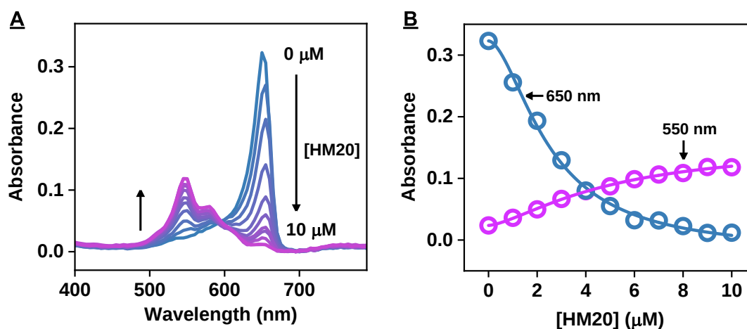
Figure S21. Binding of MTC to HM20. (A) Absorbance spectra of solutions containing 2.5 μM MTC with 0, 1, 2, 3, 4, 5, 6, 7, 8, 9 or 10 μM HM20, where the blue-to-purple color gradient shows increasing aptamer concentrations. (B) Absorbance of MTC dimers at 550 nm and J-aggregates at 650 nm plotted against the concentration of HM20.
