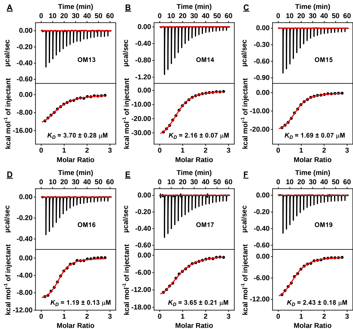
Figure S18. Characterization of oxycodone binding affinity of six aptamer candidates using ITC. The top panels display the heat generated from each titration of oxycodone into (A) OM13, (B) OM14, (C) OM15, (D) OM16, (E) OM17 and (F) OM19. Bottom panels show the integrated heat of each titration after correcting for the heat of dilution of the titrant.
