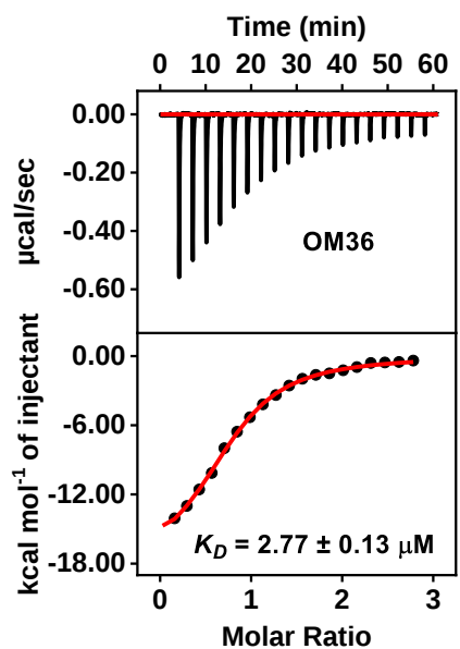
Figure S20. Characterization of oxycodone binding affinity of aptamer candidate OM36 using ITC. The top panel displays the heat generated from each titration of oxycodone into OM36. Bottom panel shows the integrated heat of each titration after correcting for the heat of dilution of the titrant.
