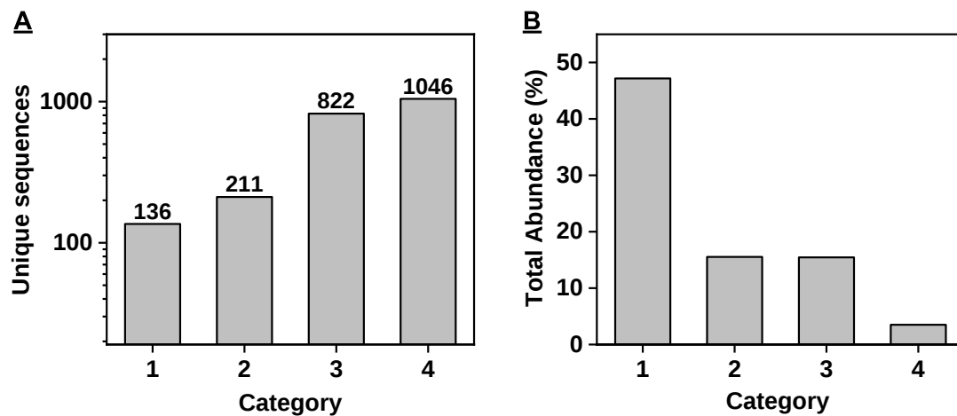
Figure S10. HTS analysis of the final T6 pool for oxycodone and oxymorphone. (A) The number of unique sequences and (B) percent of total pool belonging to each of the four categories described in the main text.
