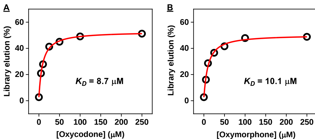
Figure S7. Binding affinity of the round T6 pool for (A) oxycodone and (B) oxymorphone. All fractions were PCR amplified and then analyzed via gel-elution assay. All binding curves were fitted with a modified one-site Langmuir equation to determine K_D .
