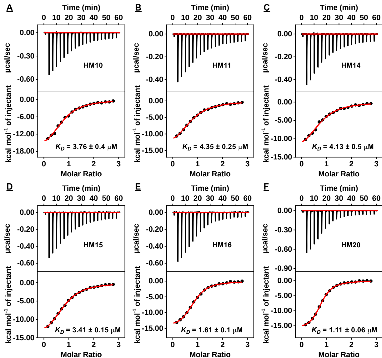
Figure S12. Characterization of morphine binding affinity of six aptamer candidates using ITC. The top panels display the heat generated from each titration of morphine into (A) HM10, (B) HM11, (C) HM14, (D) HM15, (E) HM16 and (F) HM20. Bottom panels show the integrated heat of each titration after correcting for the heat of dilution of the titrant.
