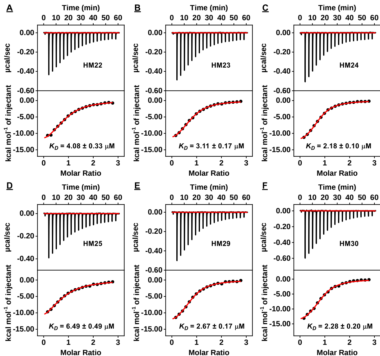
Figure S13. Characterization of morphine binding affinity of six aptamer candidates using ITC. The top panels display the heat generated from each titration of morphine into (A) HM22, (B) HM23, (C) HM24, (D) HM25, (E) HM29 and (F) HM30. Bottom panels show the integrated heat of each titration after correcting for the heat of dilution of the titrant.
