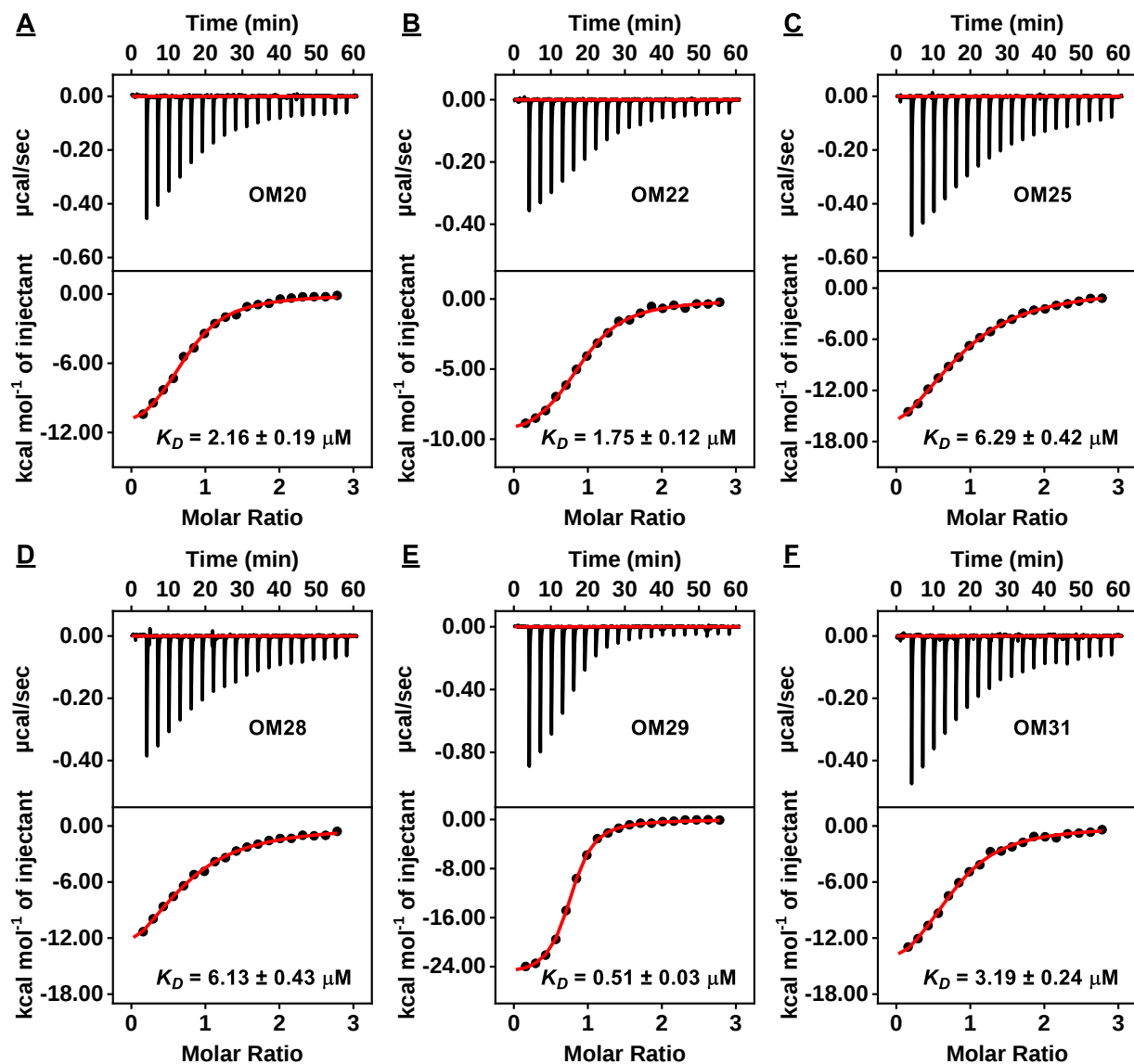
Figure S19. Characterization of oxycodone binding affinity of six aptamer candidates using ITC. The top panels display the heat generated from each titration of oxycodone into (A) OM20, (B) OM22, (C) OM25, (D) OM28, (E) OM29 and (F) OM31. Bottom panels show the integrated heat of each titration after correcting for the heat of dilution of the titrant.
