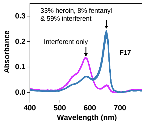
Figure S25. Absorbance spectra of F17-MTC complexes in the presence of a mixture of heroin, fentanyl, and interferent (caffeine, lidocaine lactose, or mannitol) as well as each interferent alone.
