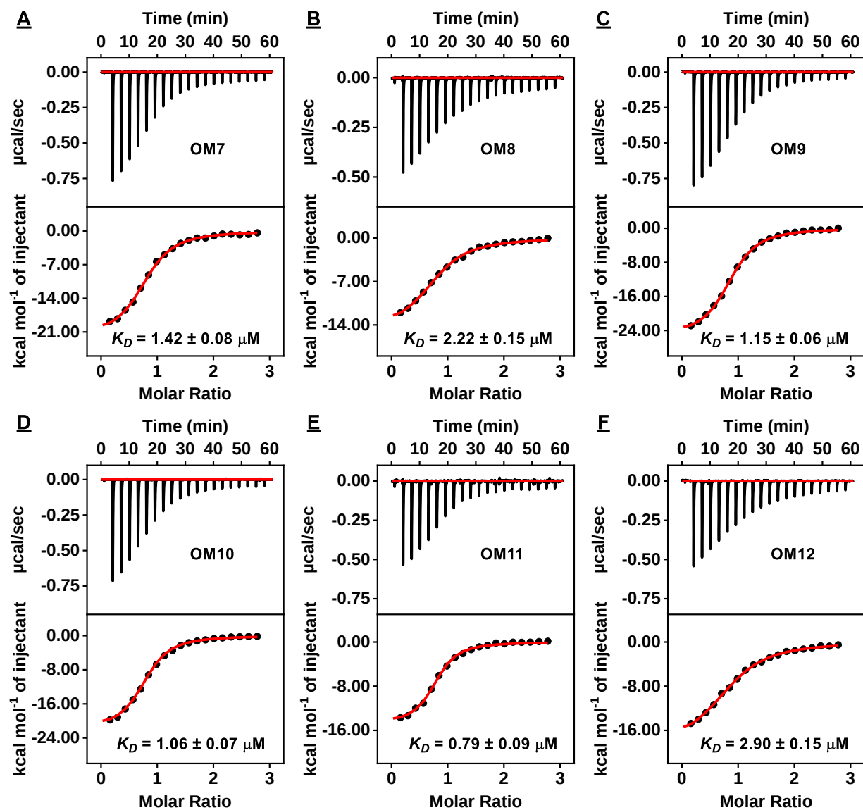
Figure S17. Characterization of oxycodone binding affinity of six aptamer candidates using ITC. The top panels display the heat generated from each titration of oxycodone into (A) OM7, (B) OM8, (C) OM9, (D) OM10, (E) OM11 and (F) OM12. Bottom panels show the integrated heat of each titration after correcting for the heat of dilution of the titrant.
