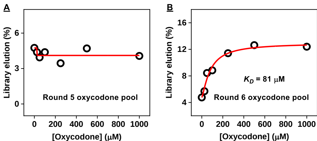
Figure S6. Binding affinity of the (A) R5 and (B) R6 pools for oxycodone. All fractions were PCR amplified and then analyzed via gel-elution assay. All binding curves were fitted with a modified one-site Langmuir equation to determine K_D .
