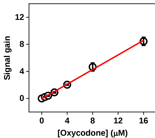
Figure S29. Linear range of detection of oxycodone using MTC and OM9.
