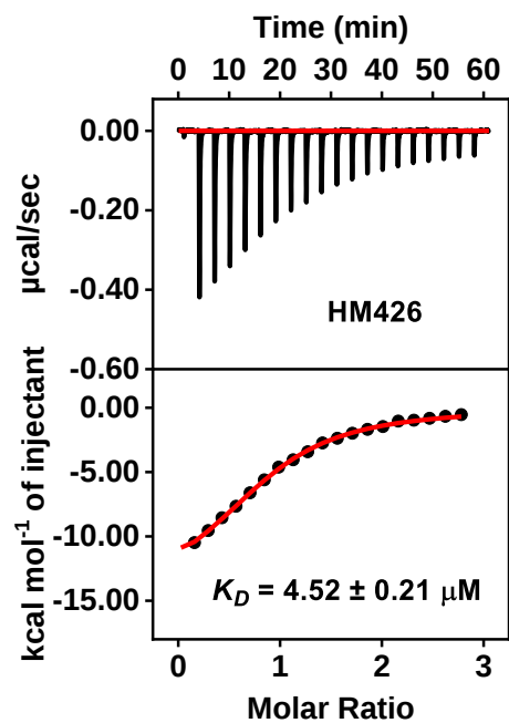
Figure S15. Characterization of morphine binding affinity of aptamer candidate HM426 using ITC. The top panel displays the heat generated from each titration of morphine into HM426. Bottom panel shows the integrated heat of each titration after correcting for the heat of dilution of the titrant.
